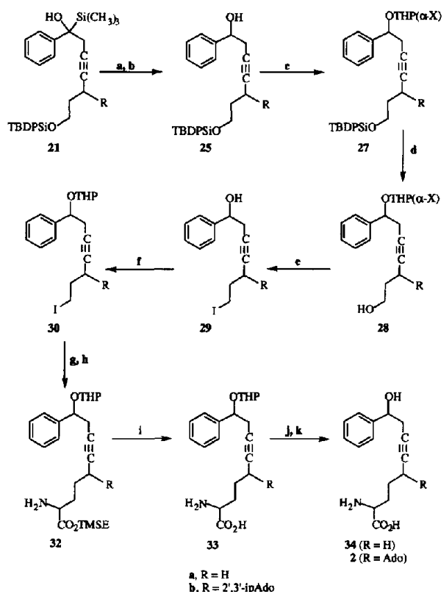
Scheme 5. Reagents: (a) KOBut, THF 0 °C; (b) HOAc in CH 2 Cl 2 , 29 82% ( 25b ); (c) 5,6-dihydro-4-methoxy-2H-pyran (X = OCH 3 ) or 5,6-dihydropyran (X = H), PPTS, CH 2 Cl 2 , 69% ( 27a ), 45% ( 27b ); (d) TBAF in THF, 91% ( 28a ), 35% ( 28b ); (e) PPh 3 , imidazole, I 2 in THF, 79% ( 29a ), 63% ( 30b ); (f) 5,6-dihydropyran, PPTS, CH 2 Cl 2 , 92% ( 30a ); (g) PhCH=NCH 2 CO 2 TMSE ( 18 ), LDA, THF/HMPA –78 °C; (h) HOAc in CH 2 Cl 2 , 56% ( 32a ), 49% ( 32b ) overall yields for two steps; (i) TBAF in THF; (j) HOAc:THF:H 2 O (4:2:1) 50 °C, 9 h; (k) anion exchange chromatography.
