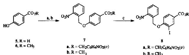
Scheme 2. Reagents: (a) NaOCH 3 (2.4 equiv, 5 → 7a ; 1.2 equiv, 6 → 7b ); (b) o -nitrobenzylbromide (2.4 equiv, 5 → 7a ; 1.2 equiv, 6 → 7b ), DMF; 66% ( 7a ), 85% ( 7b ); (c) AgTFA, CH 2 Cl 2 , 1, 49% ( 8a ), 92% ( 8b ).
