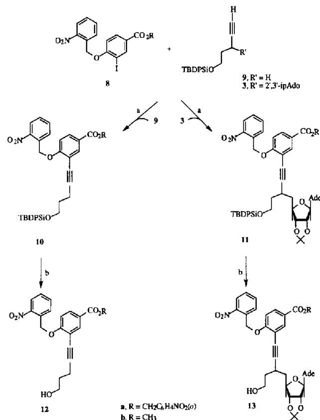
Scheme 3. Reagents: (a) PdCl 2 (PPh 3 ) 2 , Et 3 N, CuI, DMF, 60% ( 10a ), 85% ( 10b ), 44% ( 11a ), 75% ( 11b ); (b) TBAF, THF/HOAc (99:1), 80% ( 12a ), 65% ( 12b ), 92% ( 13a ), 99% ( 13b ).
