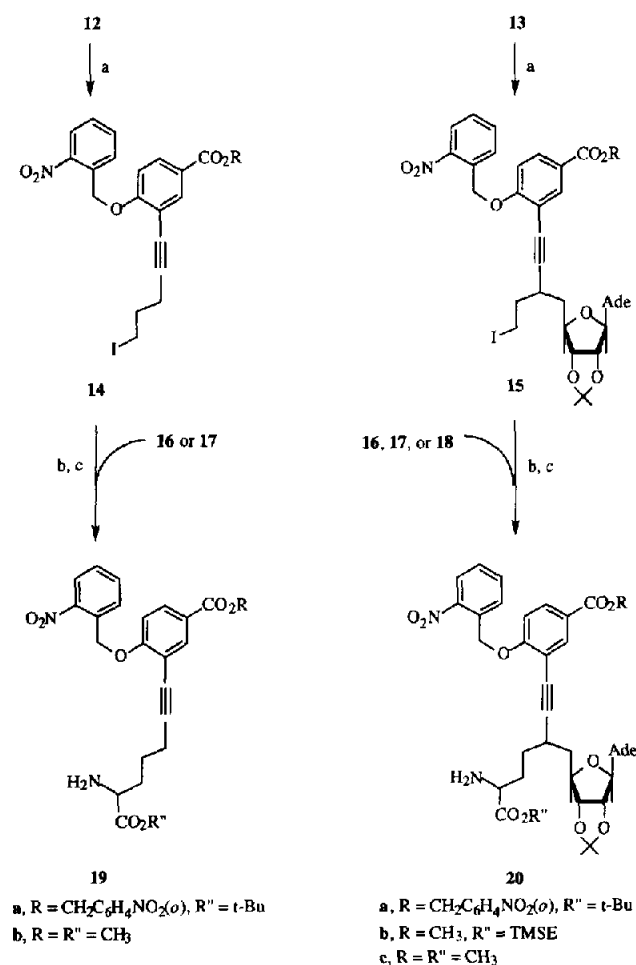
Scheme 4. Reagents: (a) (PhO) 3 P + CH 3 I, CH 2 Cl 2 , 79% ( 14a ), 70% ( 15a ), 84% ( 15b ); (b) PhCH=NCH 2 CO 2 R'' ( 16 , R'' = CH 3 ; 17 , R'' = t -Bu; 18 , R'' = TMSE), LDA, THF/HMPA (9:1); (c) 80% HCO 2 H, 19a , or HOAc/CH 2 Cl 2 (<1%), 20a,c , 33% ( 19a ), 68% ( 20a ), 56% ( 20c ).
